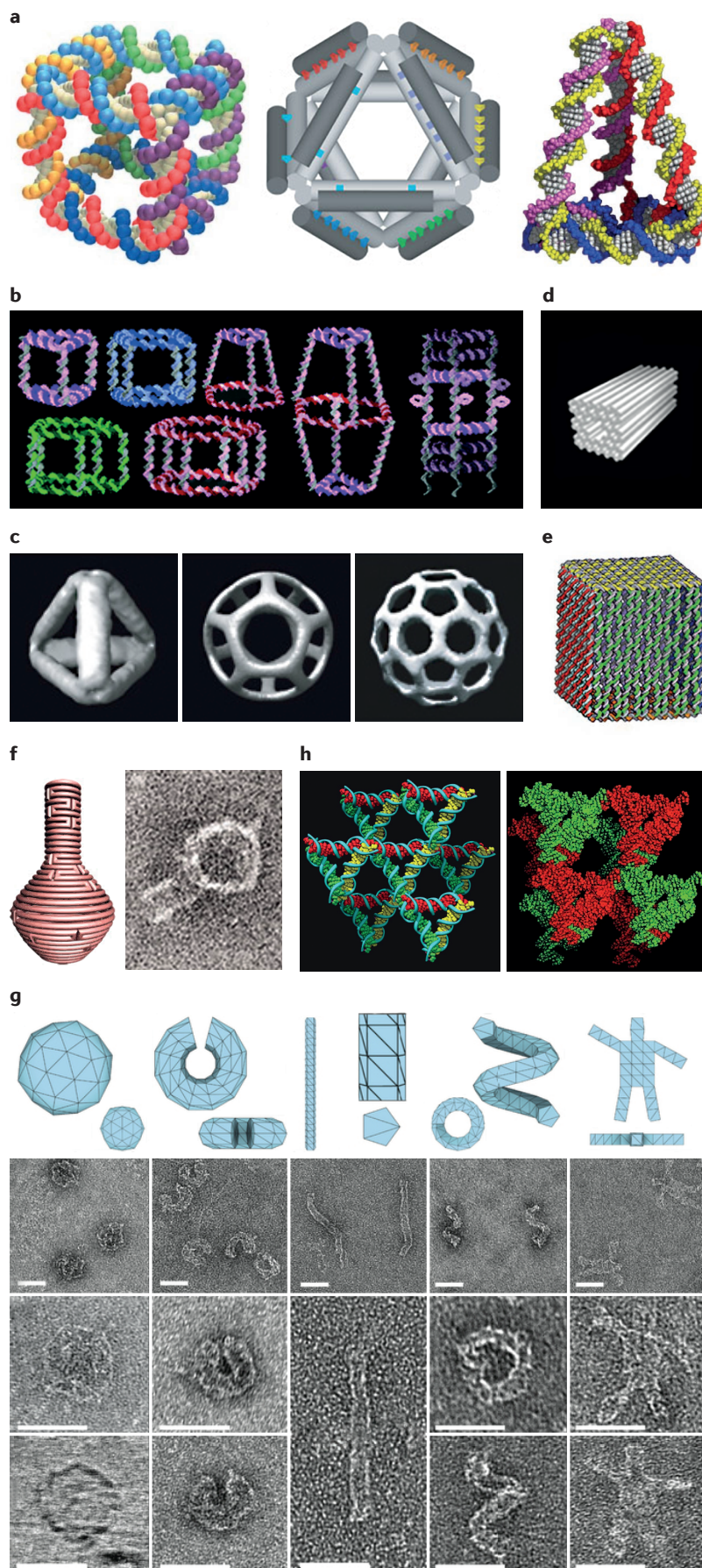
Figure 4 | Three-dimensional structures from DNA.
