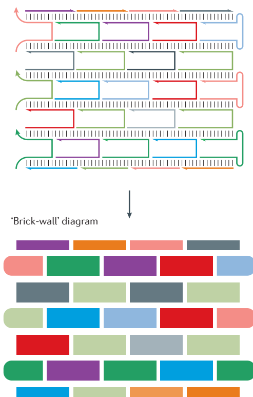
Figure 3 | DNA origami and single-stranded tile assembly. a Scaffolded DNA origami. The left panel shows a long genomic DNA strand folded with the help of small staple strands to give a desired, computationally designed shape. The right panels show atomic force microscopy (AFM) images of DNA origami shapes. Scale bars are 100 nm unless noted otherwise 25 . b Single-stranded tile assembly. The left panel shows single strands of DNA containing four domains that are computationally designed to associate into staggered duplexes, resulting in DNA lattices. The right panel shows AFM images of single-stranded tile assemblies 27 . Panel a is adapted with permission from REF. 25, Macmillan Publishers Limited. Panel b is adapted with permission from REF. 27, Macmillan Publishers Limited.
